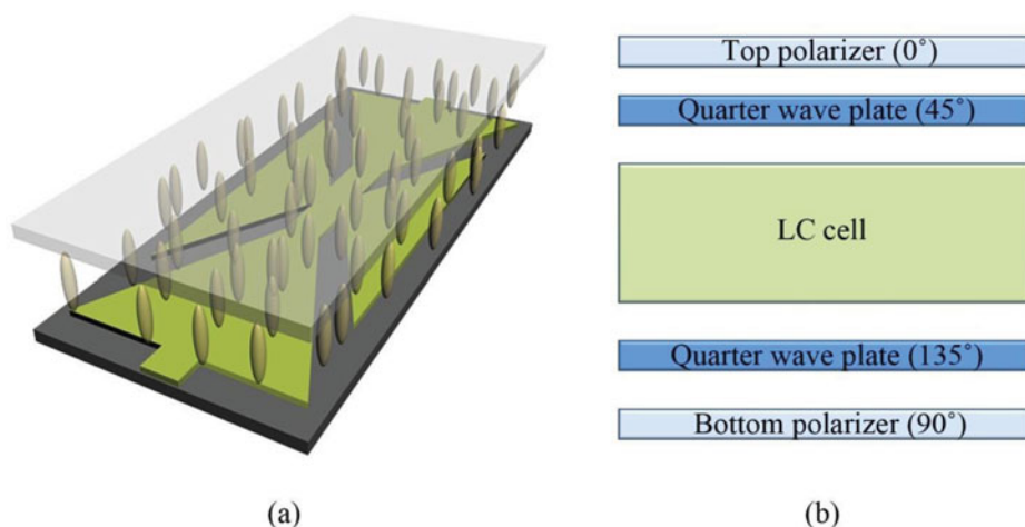
Figure 1. Electrode configurations of the proposed (a) x-shaped electrode and (b) cell structure for the optical compensation.
