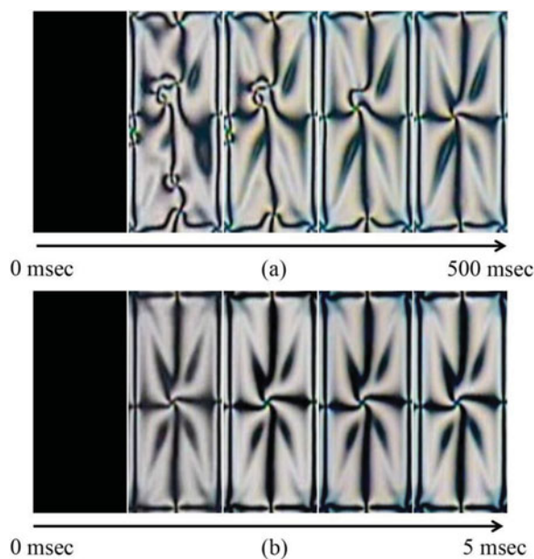
Figure 4. The time-resolved microscopic textures (a) for using only vertical alignment material and (b) for using mixed alignment material with RM.
