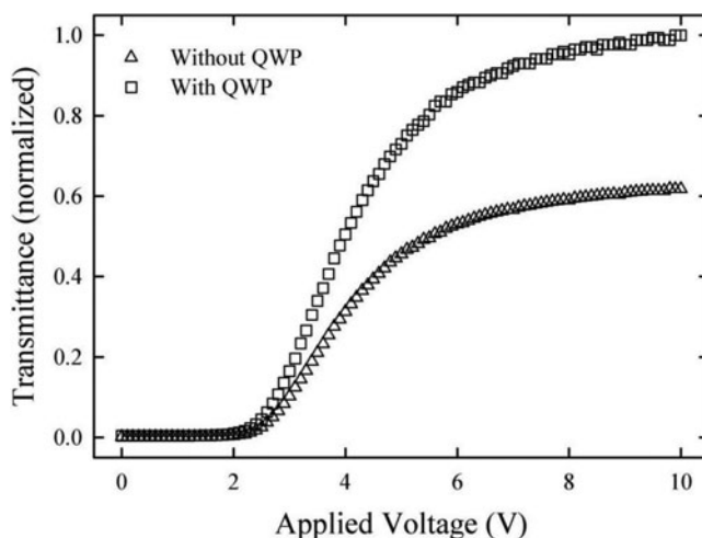
Figure 3. EO transmittances of the sample (a) without and (b) with QWPs.
