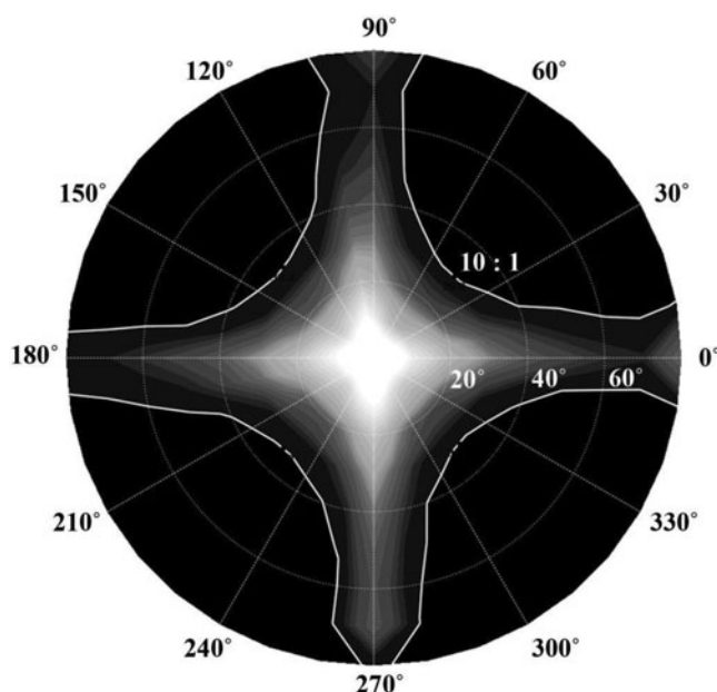
Figure 5. Measured viewing angle characteristics of the fabricated LC cell.
